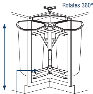
RRC28PT-W model includes hardware to mount to revolving cabinet door
