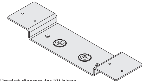
Bracket diagram for KV hinge
